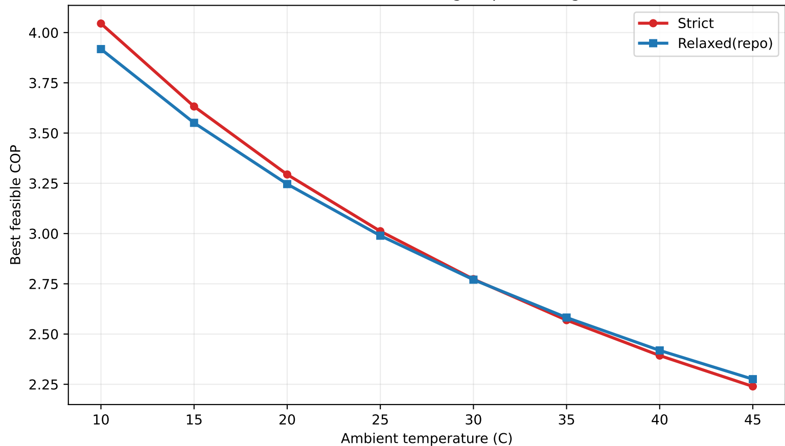
COP vs Ambient for (subcooling, superheating) = (1,3)
