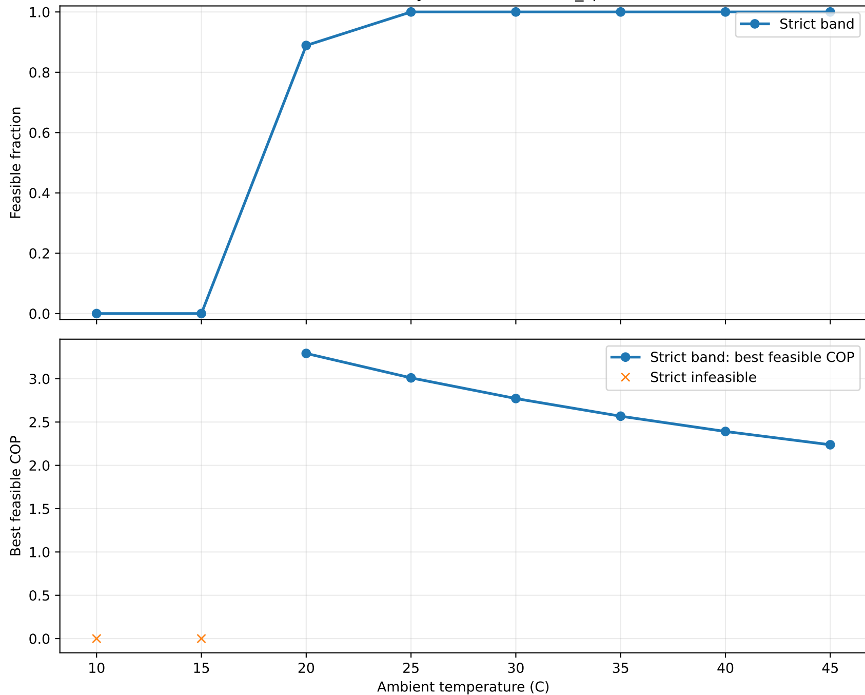
R134a PLR Feasibility Demonstration ( T_{sp} = -20\text{ C} )
