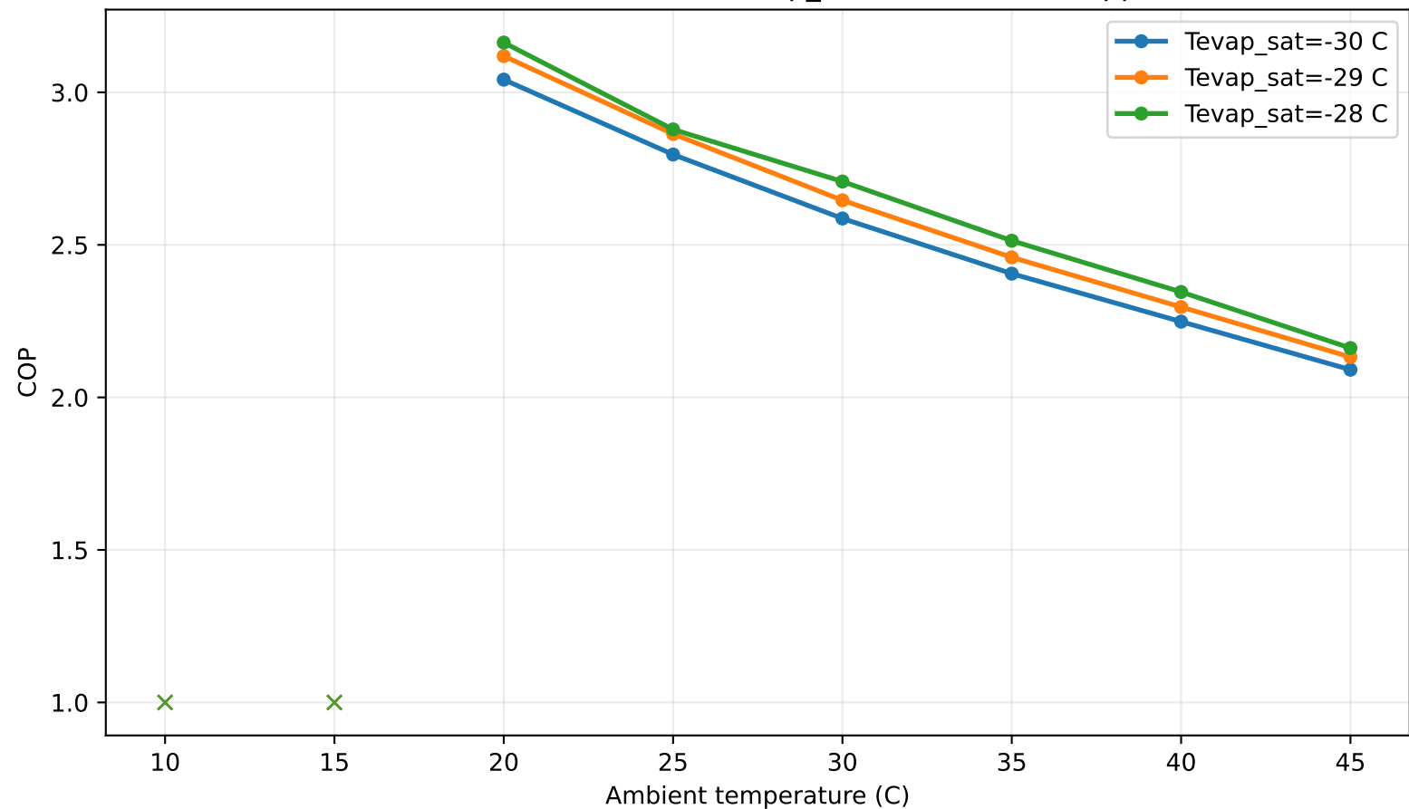
Strict band (3,3): COP vs Ambient\nTevap_sat in [-30,-28] C, approach=10 C
