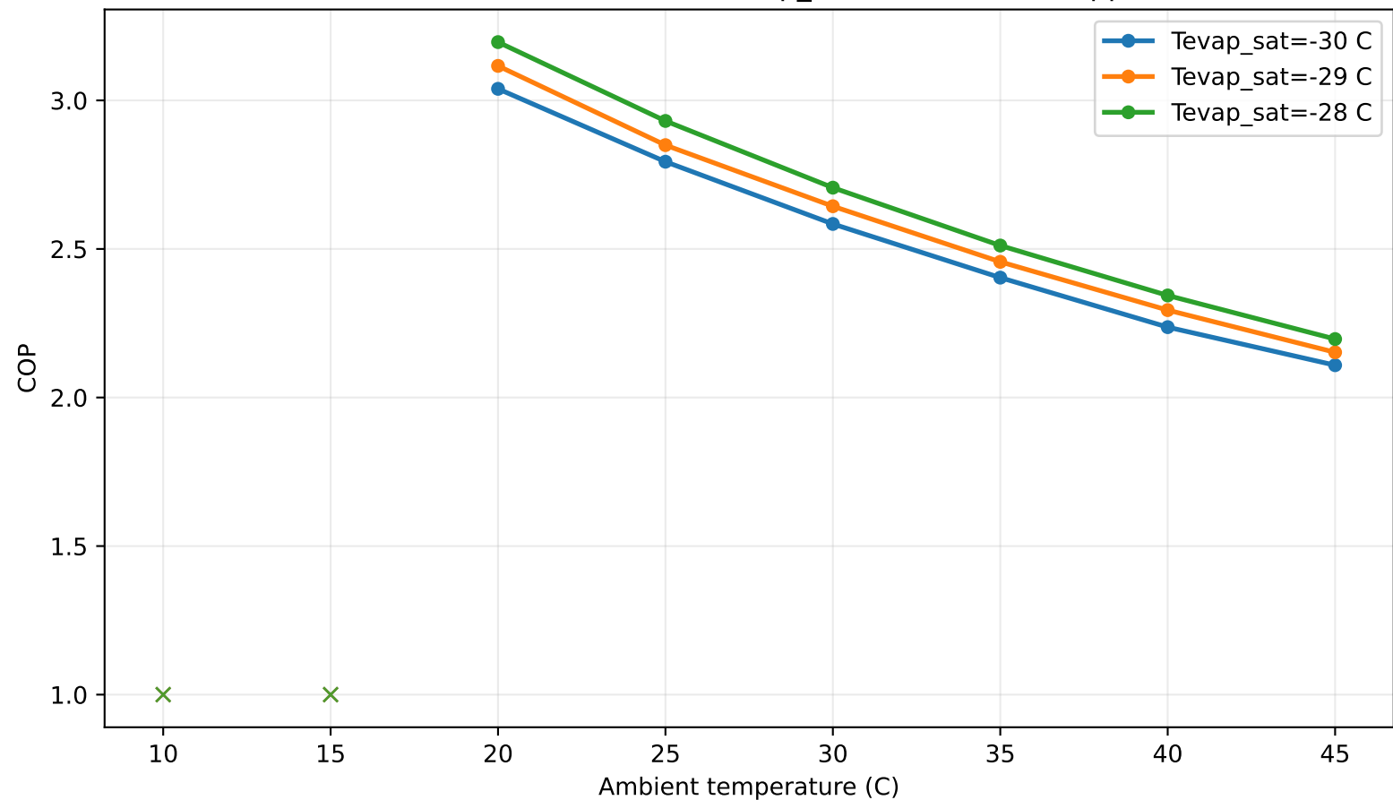
Strict band (3,5): COP vs Ambient Tevap_sat in [-30,-28] C, approach=10 C
