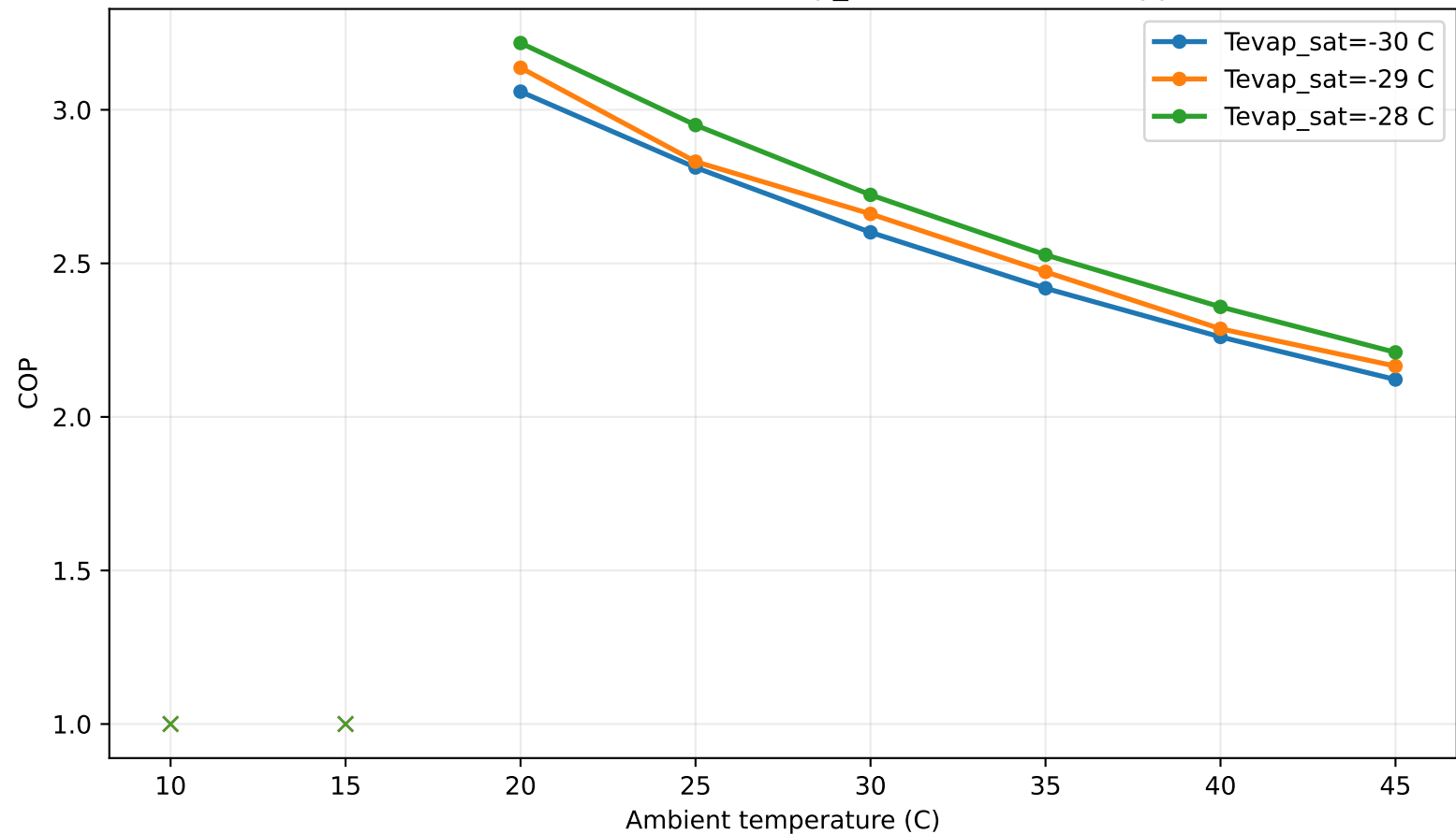
Strict band (5,7): COP vs Ambient Tevap_sat in [-30,-28] C, approach=10 C
