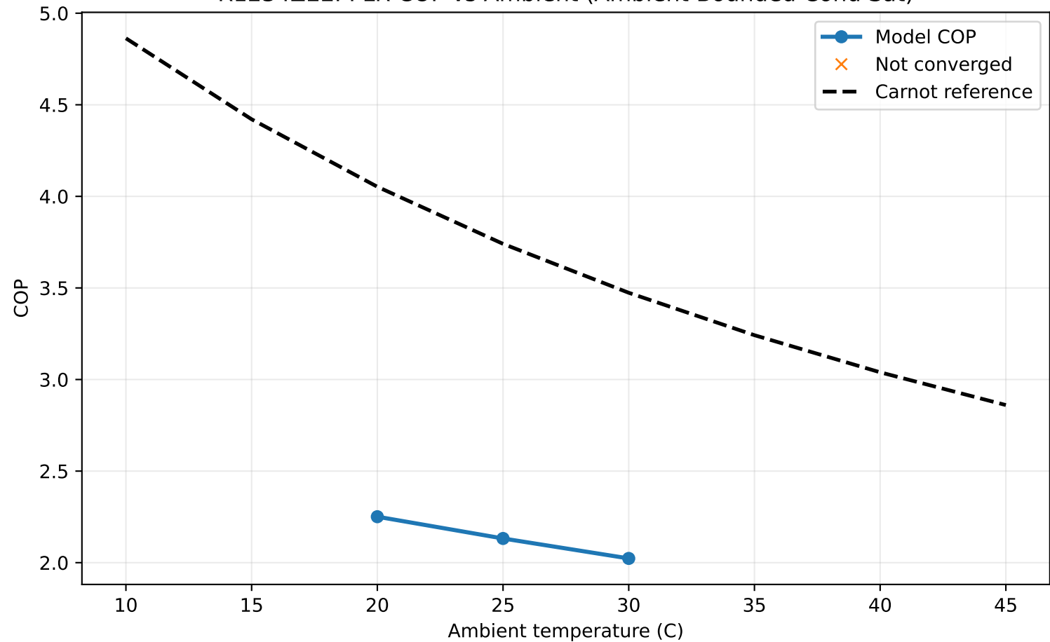
R1234ZEE: PLR COP vs Ambient (Ambient-Bounded Cond Sat)
