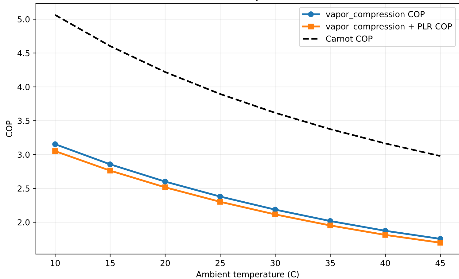
R1234ze: COP Overlay (Same Run Grid)
