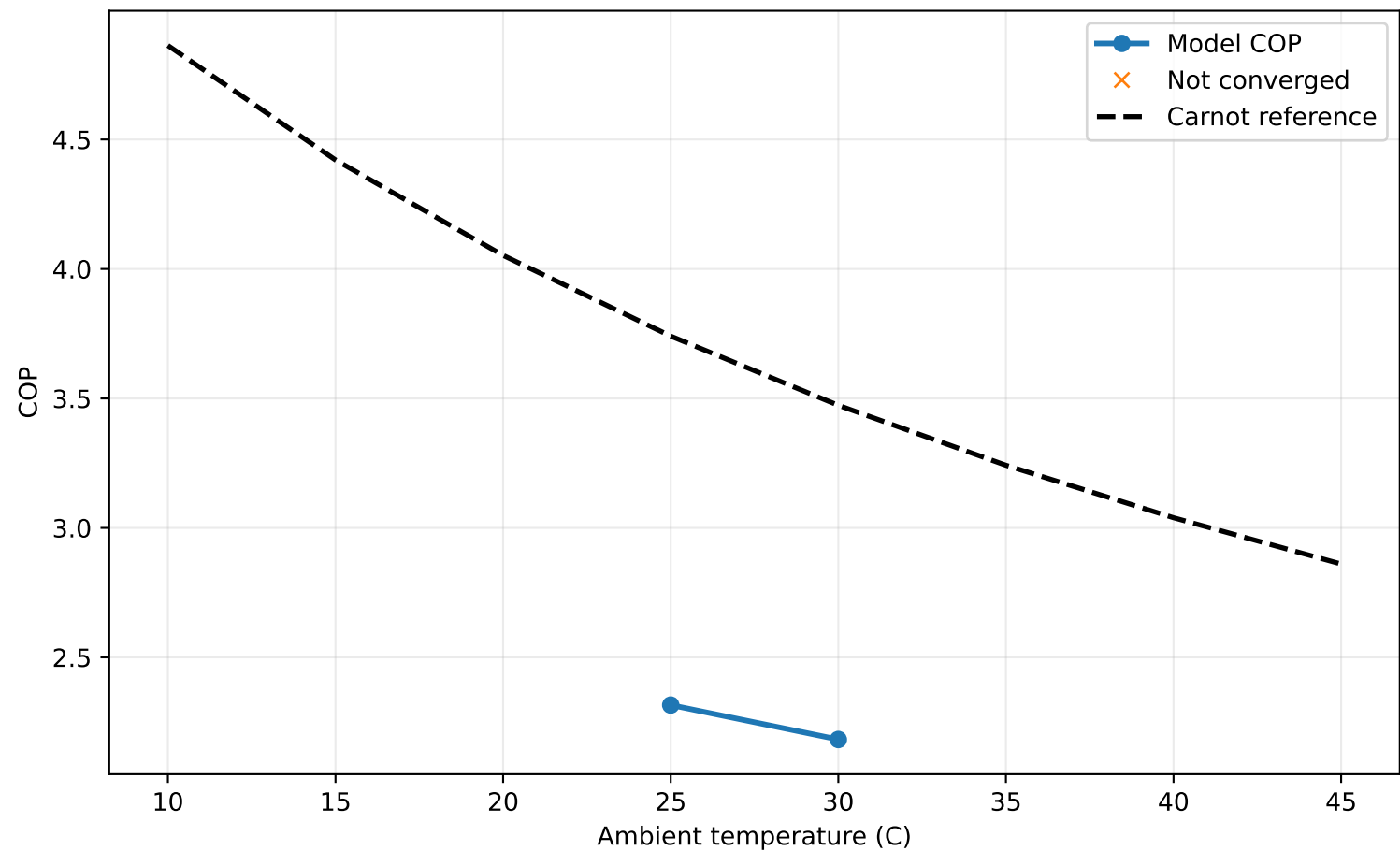
R134a: PLR COP vs Ambient (Ambient-Bounded Cond Sat)
