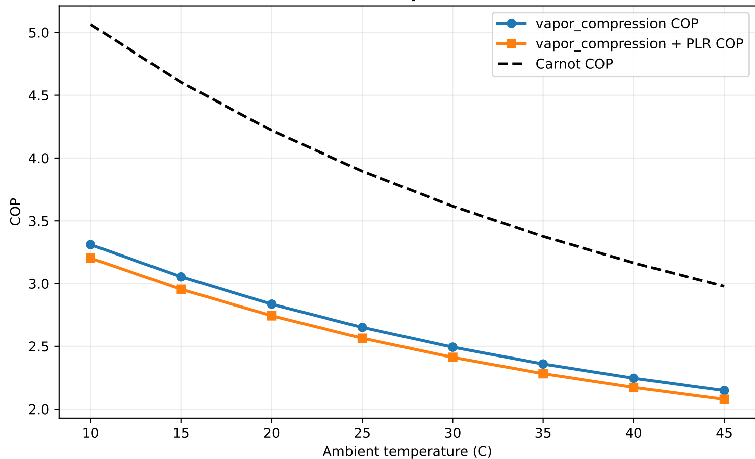
R134a: COP Overlay (Same Run Grid)
