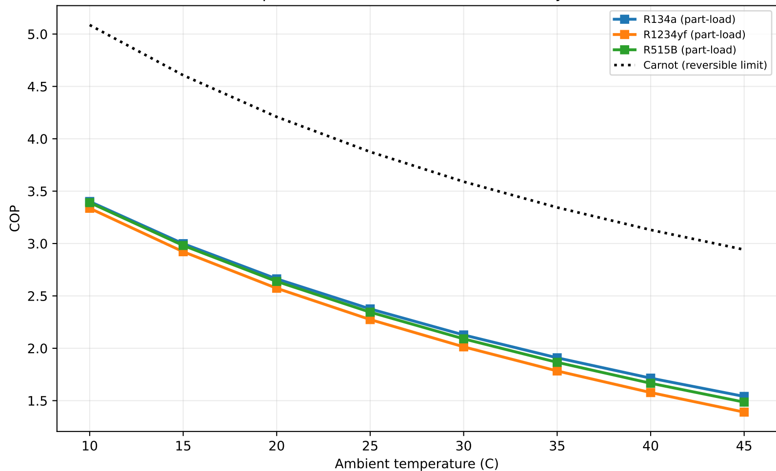
PLR benchmark (sequential warm-start): R134a vs R1234yf vs R515B vs Carnot
