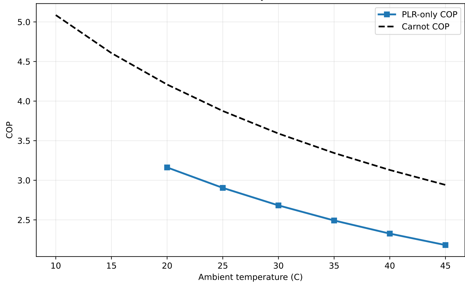
R134a: IDAES PLR-only COP vs Ambient
