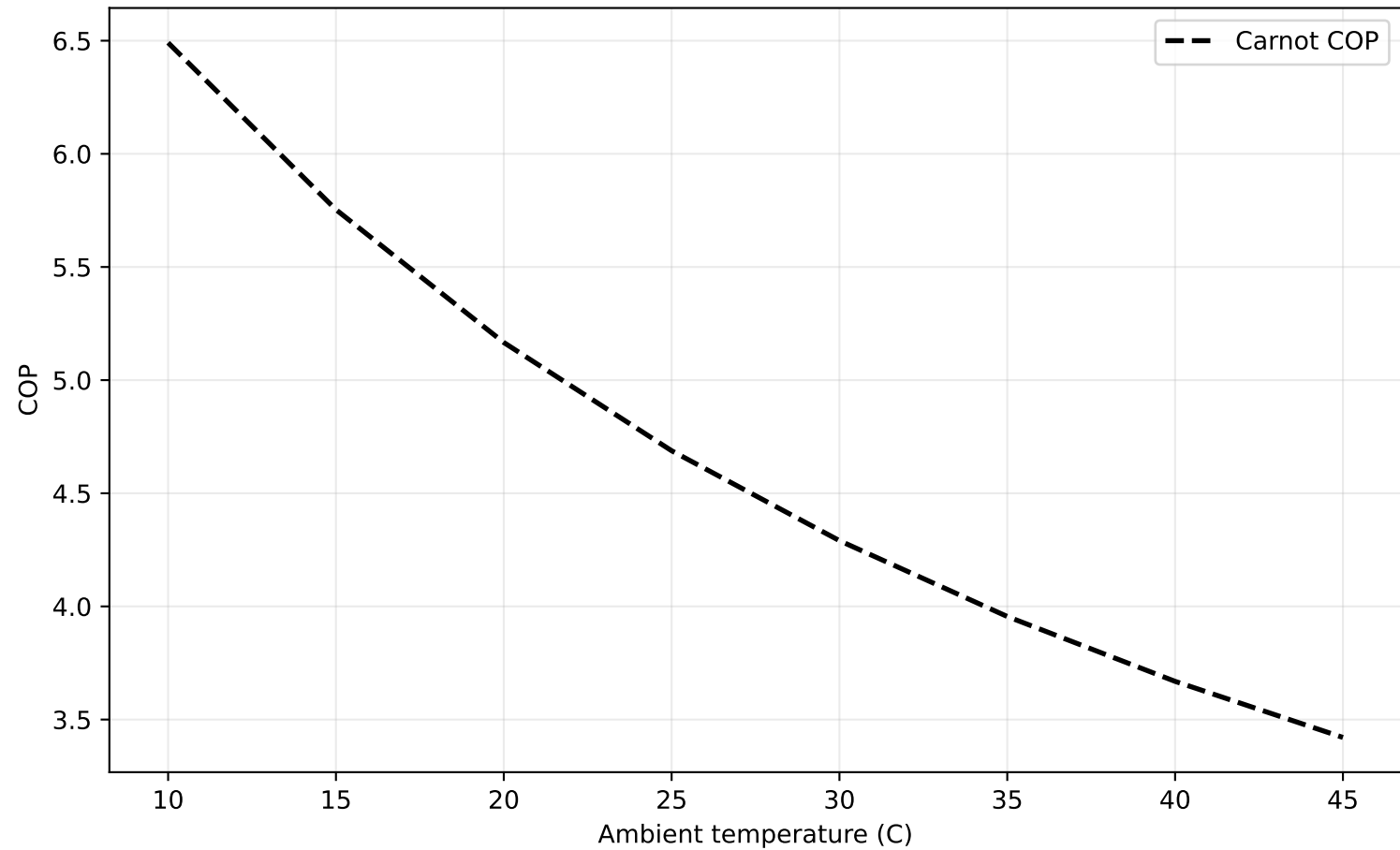
R134a: IDAES HX1D PLR + HX vs Carnot
