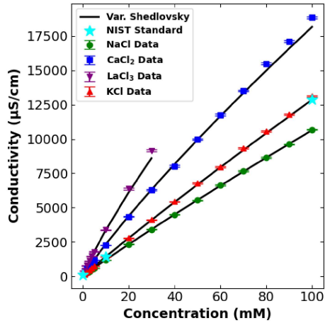
(e) Variant Shedlovsky model prediction of the calibrated conductivity data
