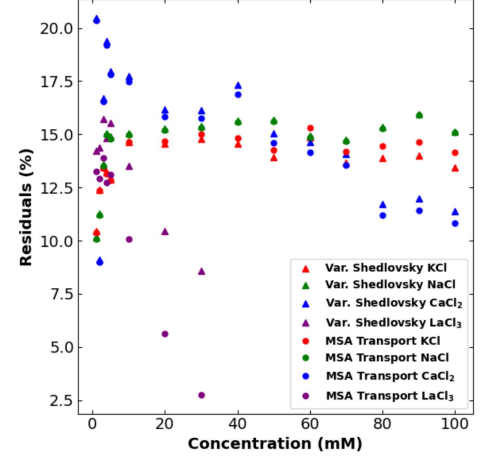
(b) Percent error of the uncalibrated conductivity data
