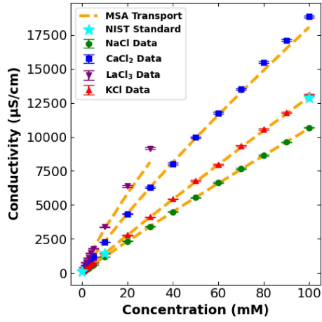
(c) MSA model prediction of the calibrated conductivity data
