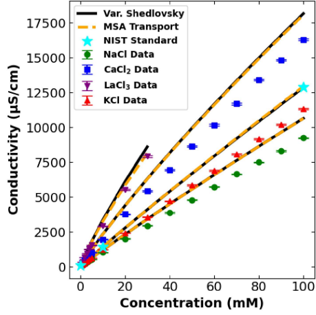
(a) Variant Shedlovsky and MSA models prediction of the uncalibrated conductivity data
