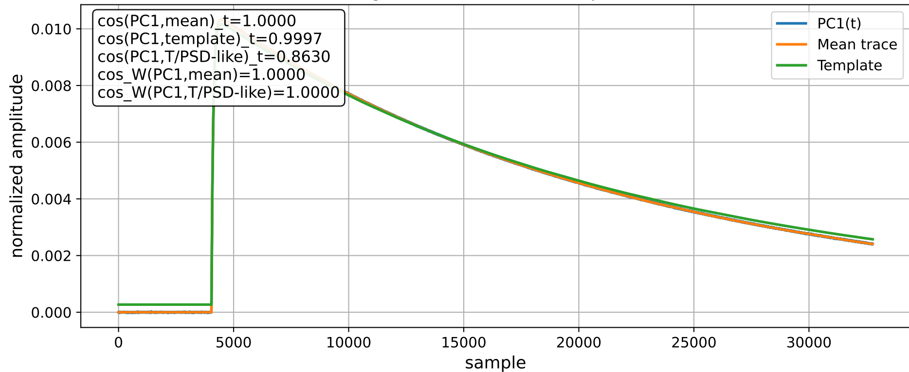
Fig.4 PC1 Vs Mean And Template
