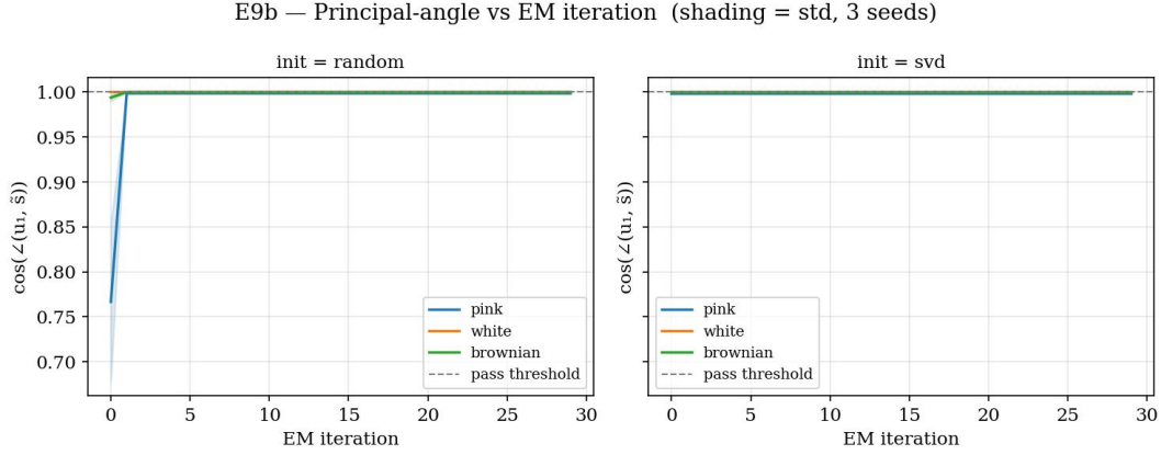
Figure 19: Principal-angle convergence over EM iterations for the same ranks and initializations as Figure 18.
