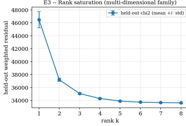
Figure 14: Held-out weighted residual \chi^2(k) versus rank on the multi-dimensional family (mean \pm std, 8 seeds).
