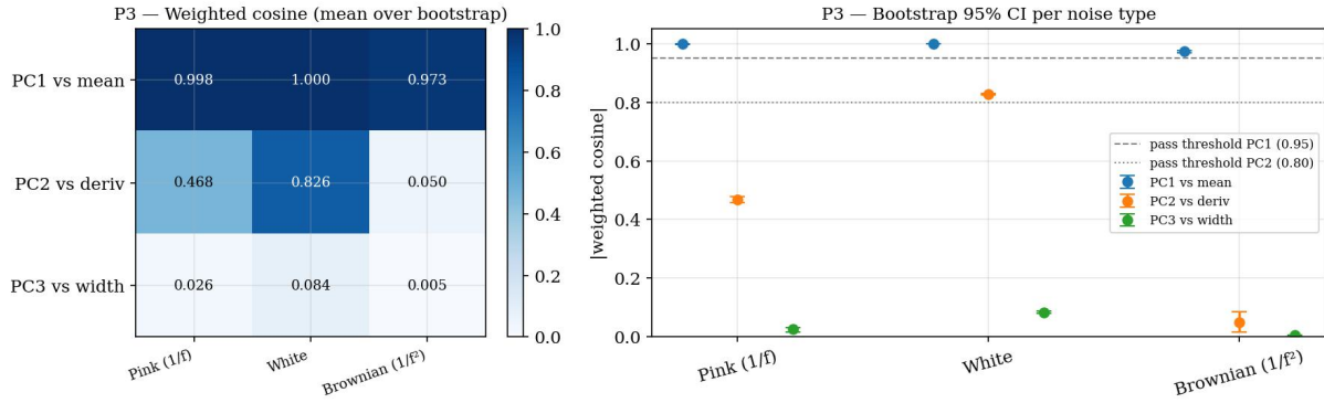
Figure 8: PC cosine score matrix: weighted cosine between each EMPCA principal component and its reference direction (mean pulse, derivative, width) for three noise types. Left: mean cosines. Right: bootstrap 95% CIs.
