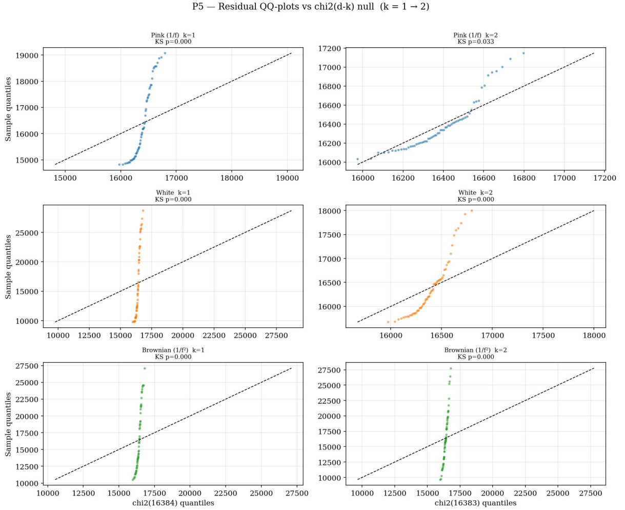
Figure 17: Residual QQ diagnostics: held-out weighted residuals against the expected \chi^2(d - k) null across ranks and noise colors.
