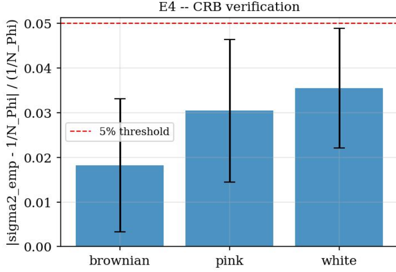
Figure 10: CRB verification: relative error between empirical amplitude variance and 1/N_{\Phi} for three noise colors; all below the 5% threshold.
