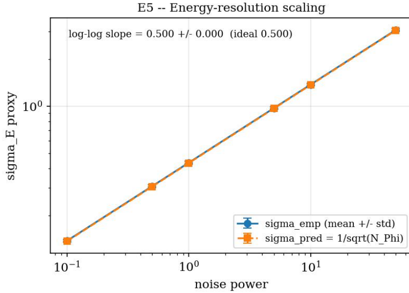
Figure 11: Energy-resolution scaling: empirical \sigma_E and the CRB prediction 1/\sqrt{N_{\Phi}} versus noise power (log-log).
