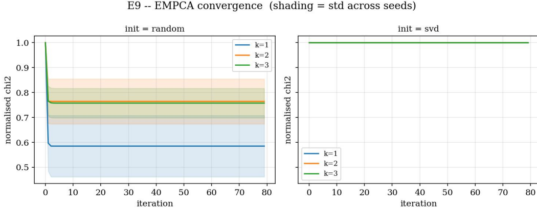
Figure 18: EMPCA convergence: normalized objective versus EM iteration for k = 1, 2, 3 under random initialization (left) and SVD warm-start (right); shaded bands = std across 8 seeds.
