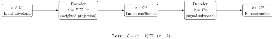
Figure 1: The noise-aware tied linear autoencoder. The encoder is the \Sigma^{-1} -adjoint of the decoder, and the training loss is the Gaussian \chi^2 objective (4).
