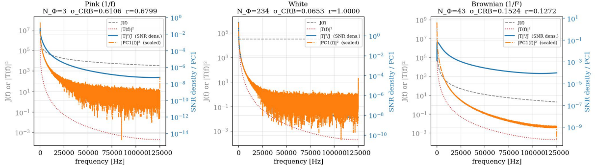
Figure 3: Experiment A, spectral view: SNR density |S(f)|^2/J(f) (blue) and learned PC1 magnitude |u_1(f)|^2 (orange, scaled) for pink, white, and Brownian noise. N_\Phi and the corresponding CRB are annotated per panel.
