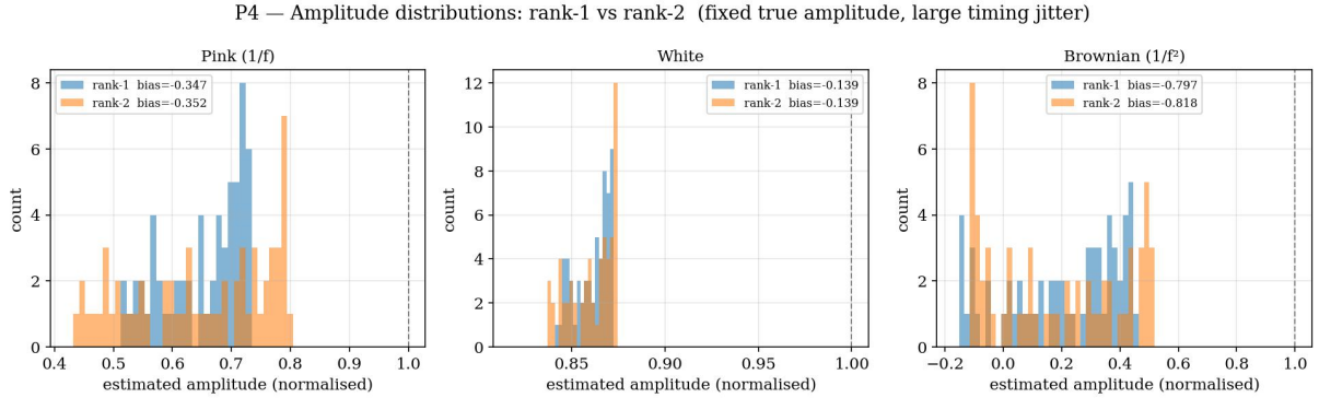
Figure 15: Amplitude distributions at rank 1 (blue) and rank 2 (orange) under large timing jitter for three noise types; dashed line = true amplitude.
