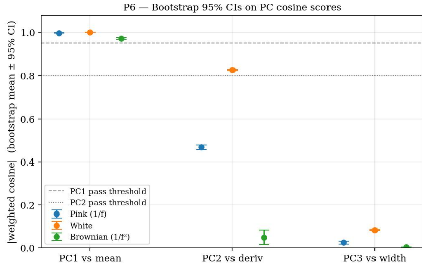
Figure 9: Bootstrap confidence intervals for the PC cosine scores, supplementary to Figure 8.
