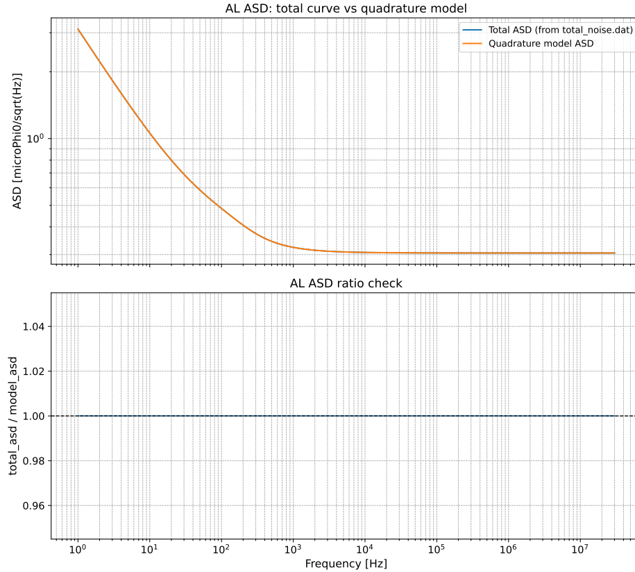
Figure 22: Study A quadrature validation: reconstructed total ASD from the component quadrature sum versus the provided total ASD.
