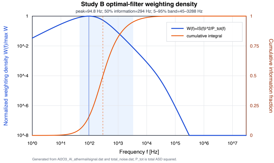
Figure 20: Optimal-filter weighting density W(f) = |S(f)|^2/P_{\text{tot}}(f) used in the noise-budget study.
