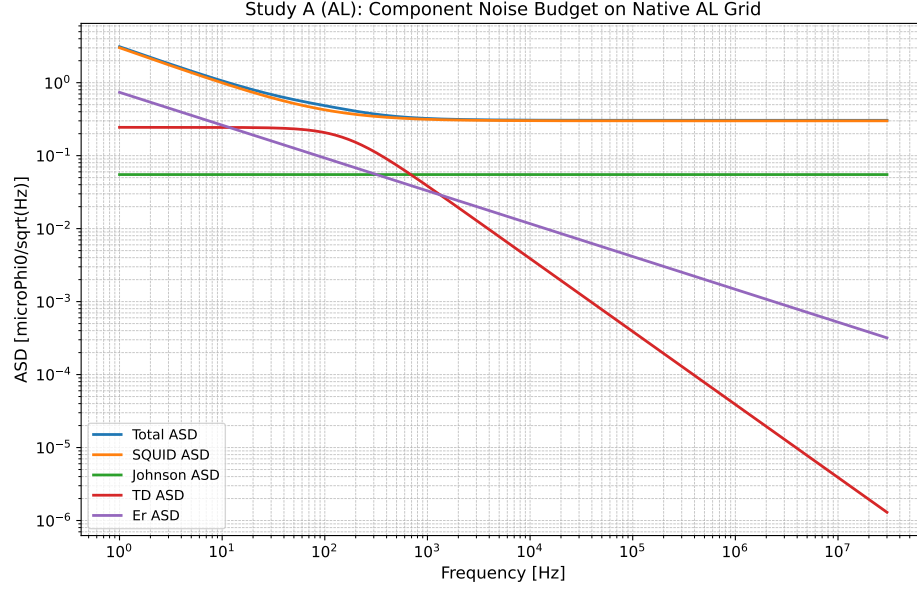
Figure 23: Study A overview of the noise budget on the native frequency grid.
