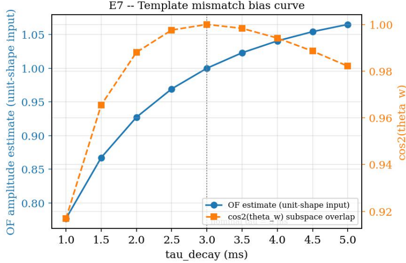
Figure 12: Template mismatch: OF amplitude estimate for a unit-amplitude signal and whitened overlap \cos^2 \theta_w versus the true decay constant; the bias follows Eq. (16).
