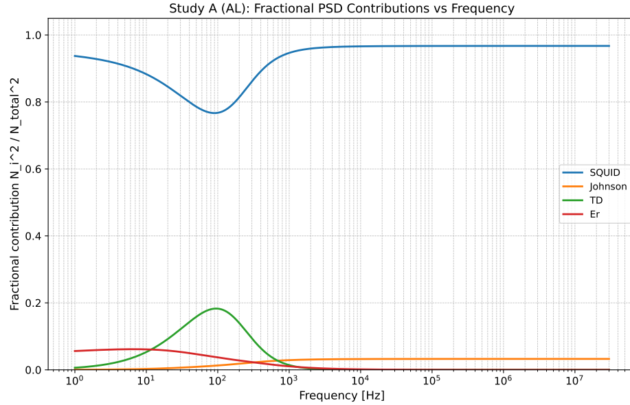
Figure 24: Fractional PSD contributions of the noise components versus frequency.
