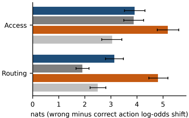
(a) Decision preference shift D_c
