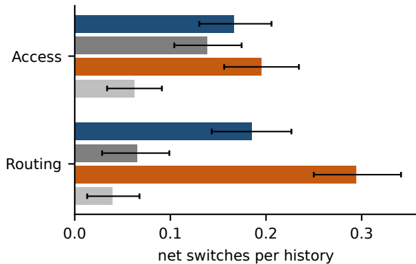
(b) Generated wrong-action switches
