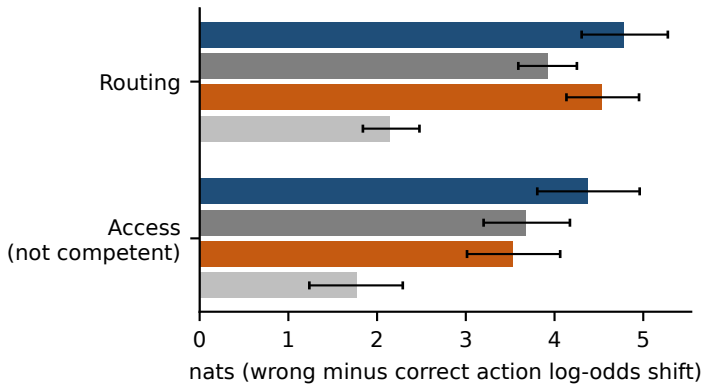
(a) Decision preference shift D_c
