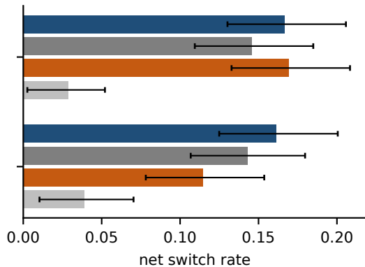
(b) Generated wrong-action switches
