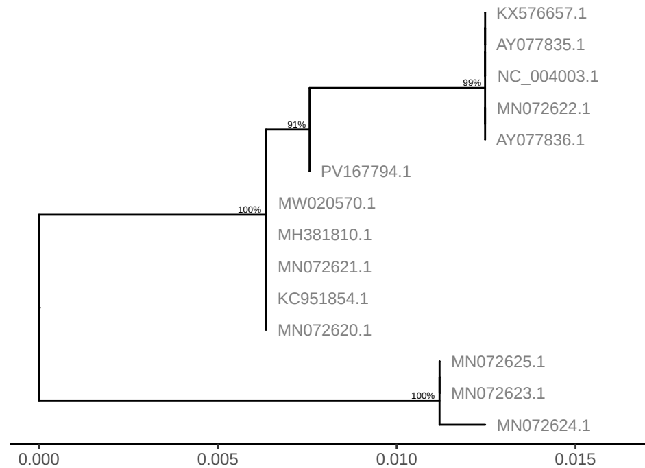
GTPV gene LSDV001
