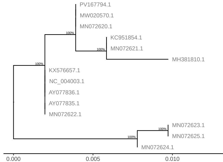
GTPV gene LSDV005
