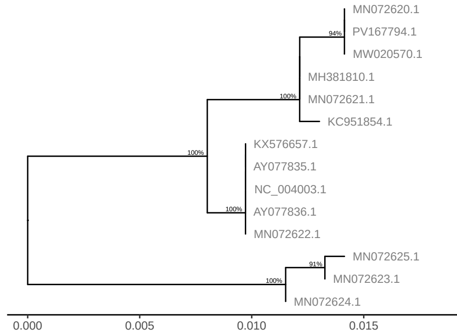
GTPV gene LSDV011
