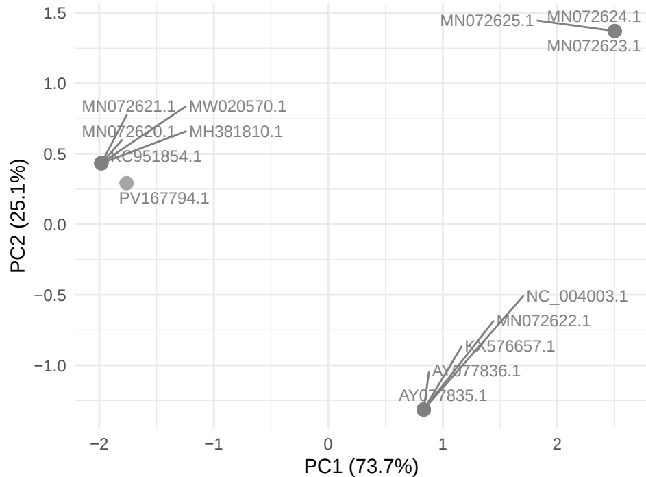
GTPV gene LSDV014
