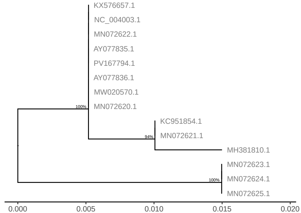
GTPV gene LSDV021
