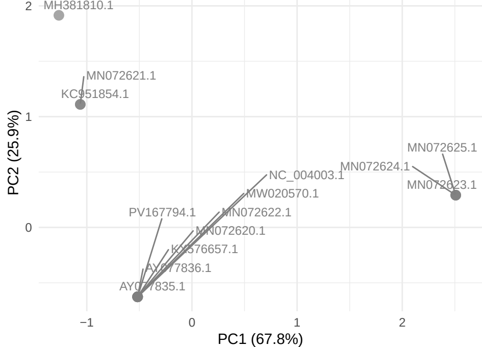
GTPV gene LSDV021
