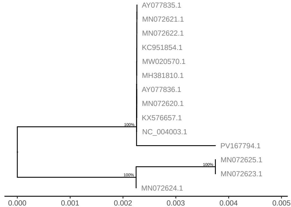
GTPV gene LSDV051
