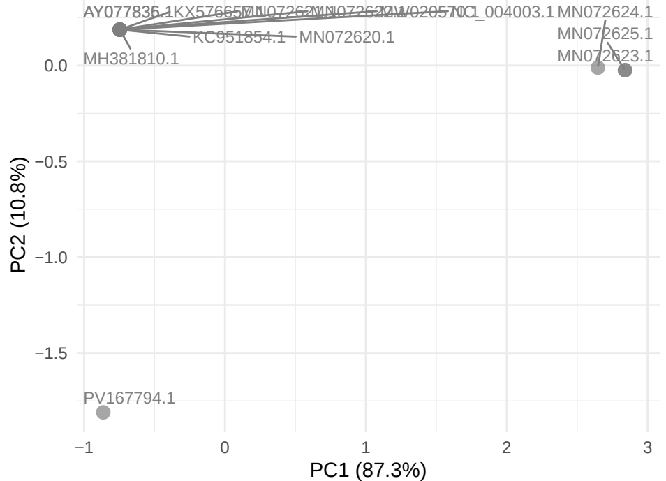
GTPV gene LSDV051
