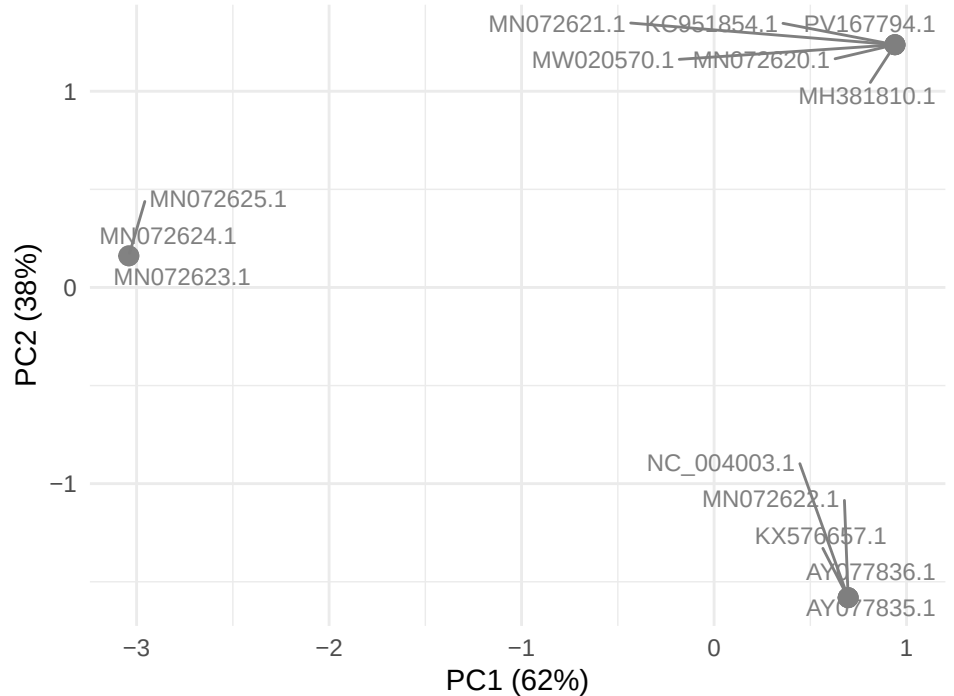
GTPV gene LSDV052
