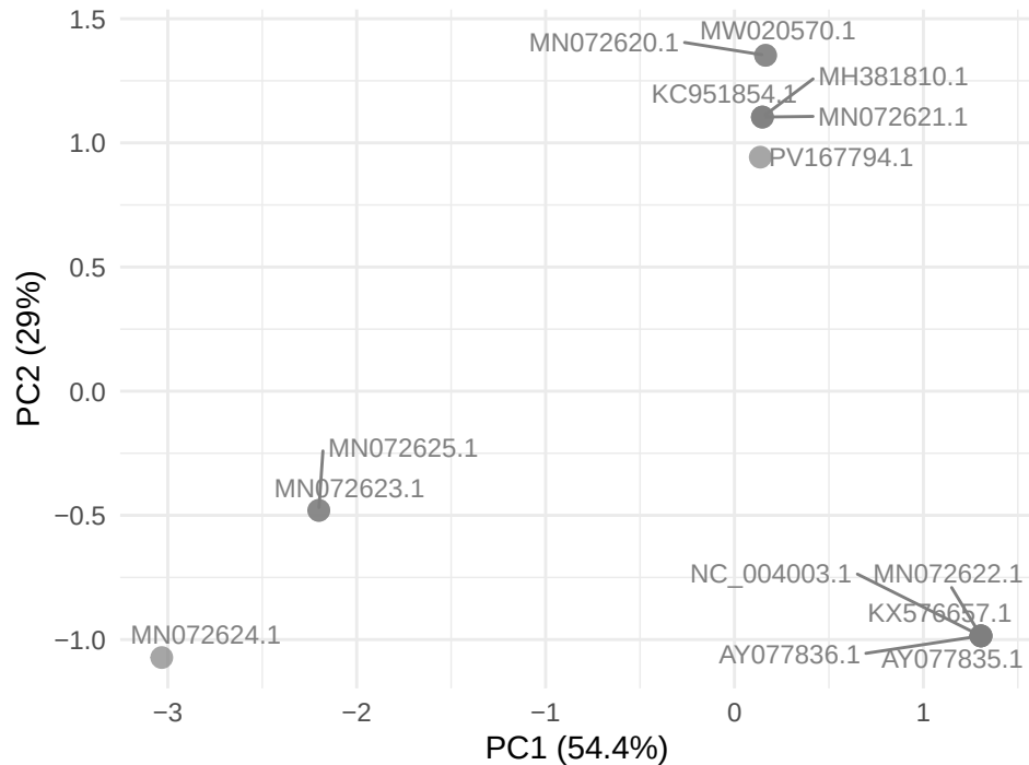
GTPV gene LSDV064
