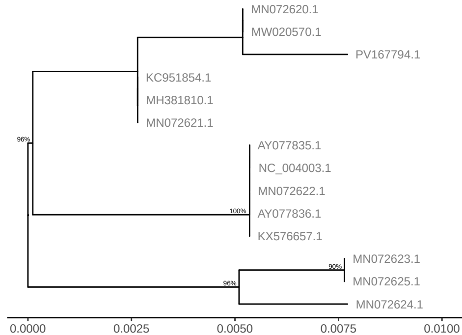
GTPV gene LSDV064
