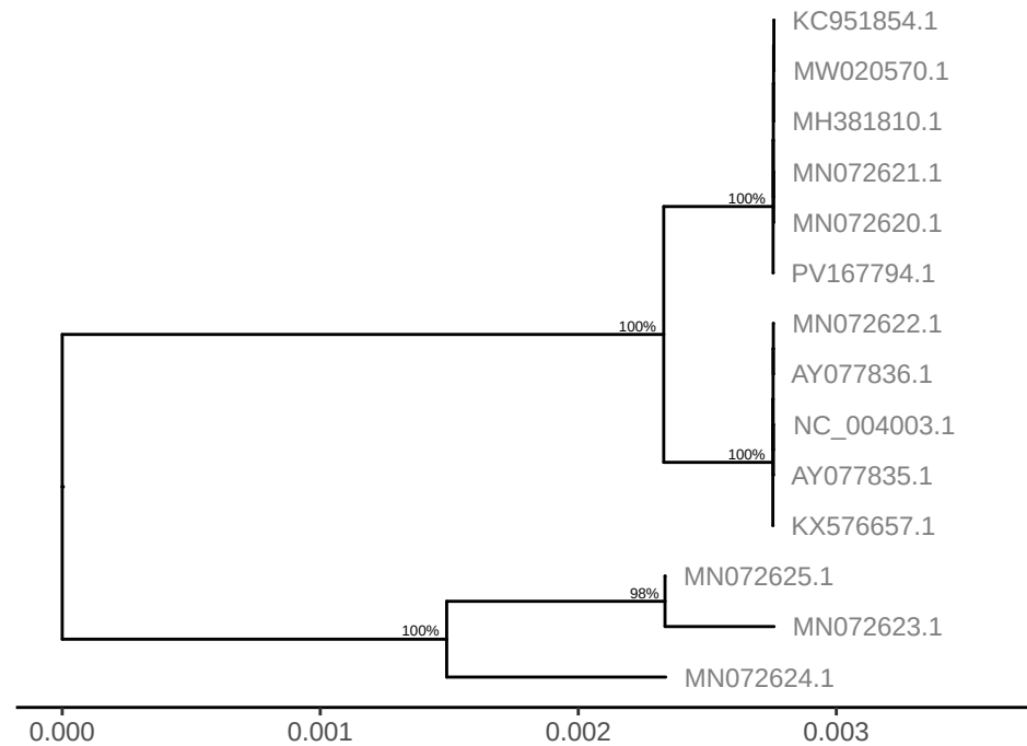
GTPV gene LSDV083
