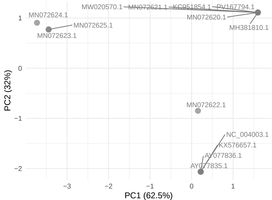
GTPV gene LSDV085
