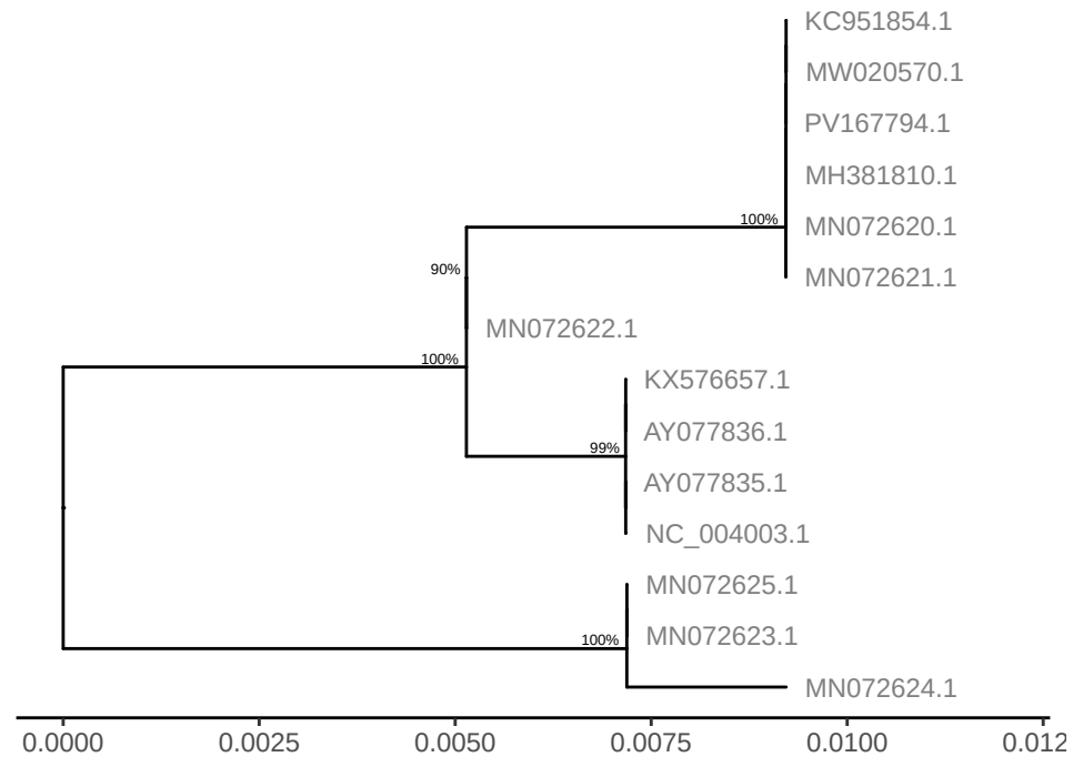
GTPV gene LSDV085
