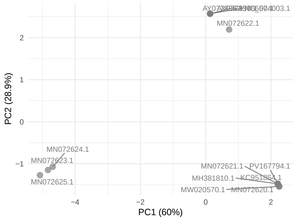
GTPV gene LSDV090
