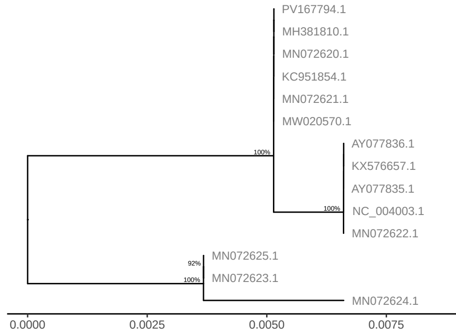
GTPV gene LSDV092
