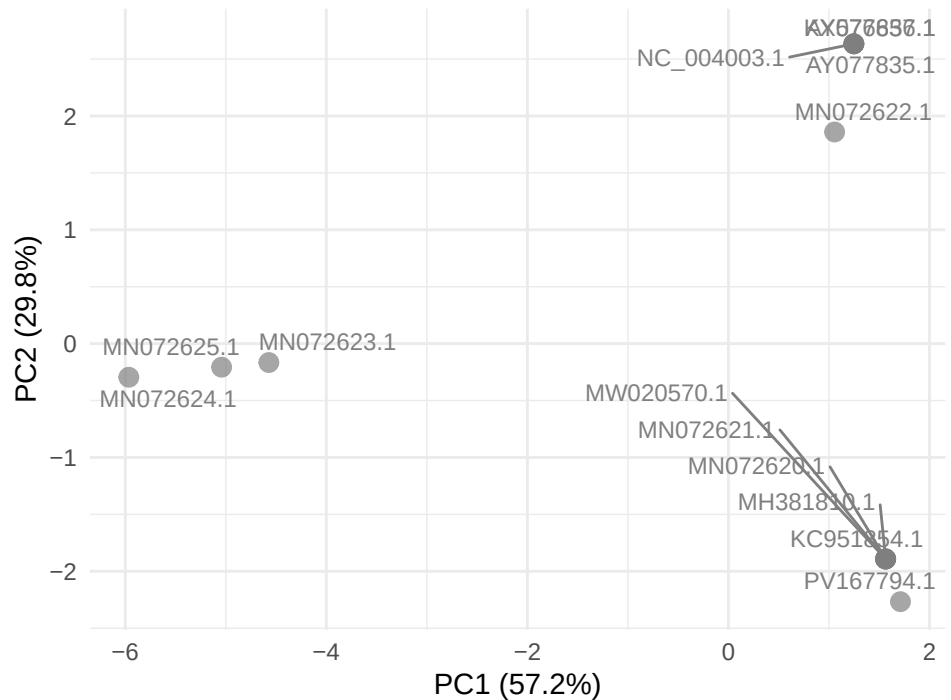
GTPV gene LSDV098
