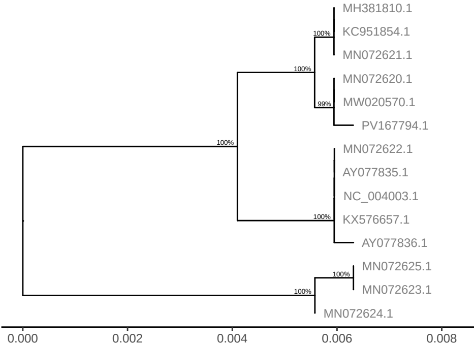
GTPV gene LSDV101
