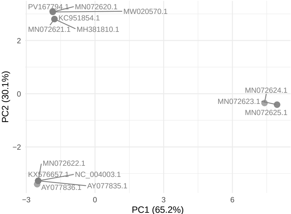
GTPV gene LSDV101
