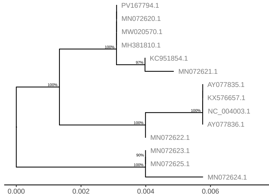
GTPV gene LSDV108
