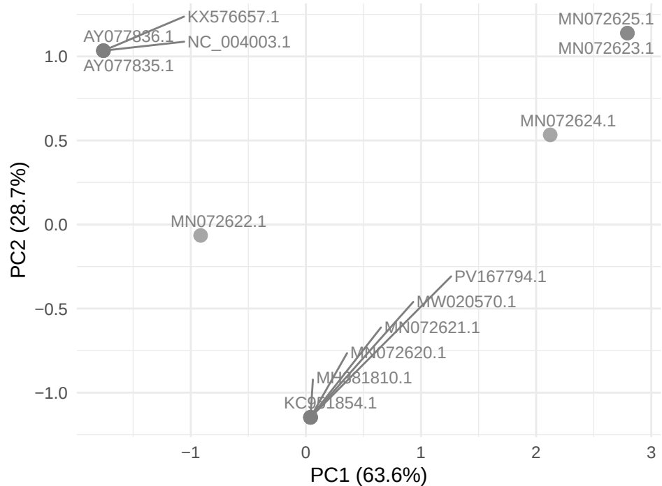
GTPV gene LSDV114
