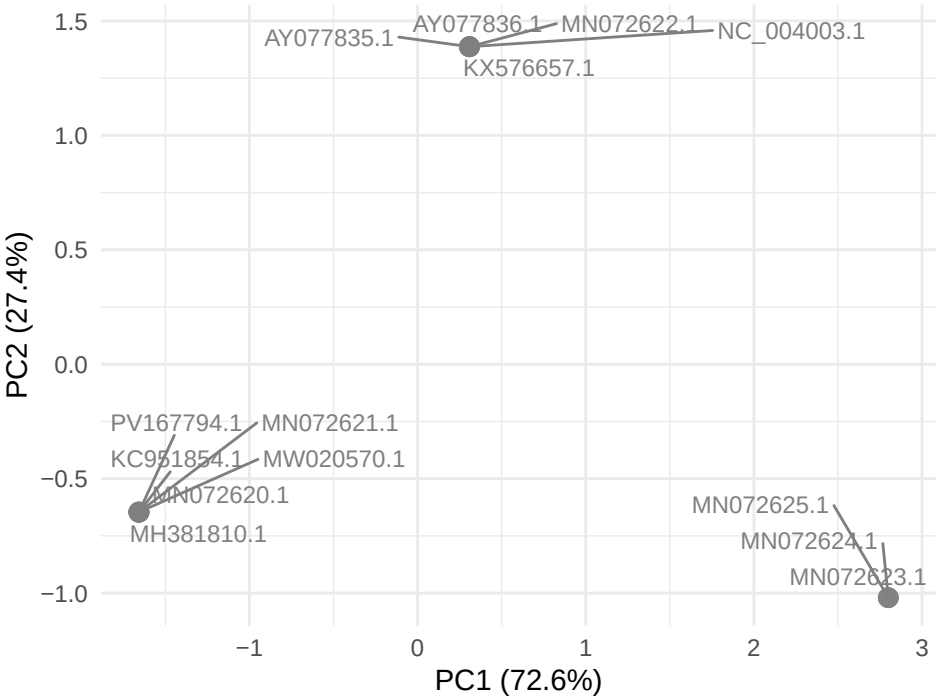
GTPV gene LSDV123
