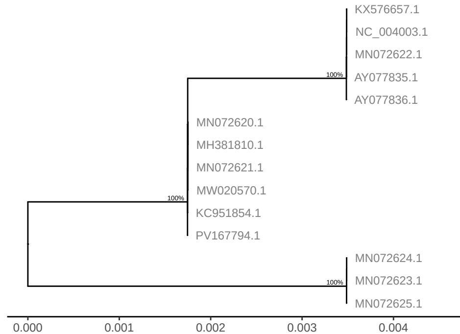
GTPV gene LSDV124
