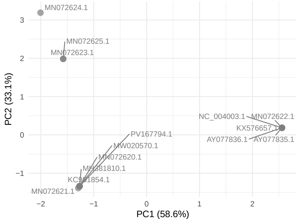
GTPV gene LSDV126
