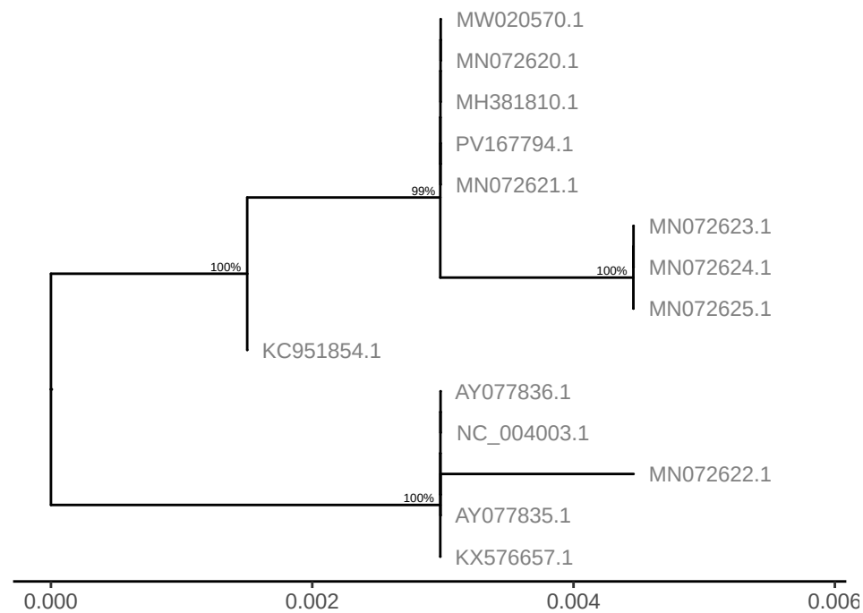
GTPV gene LSDV141
