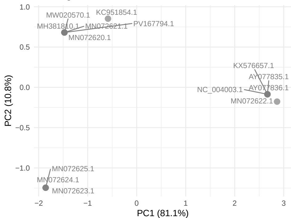
GTPV gene LSDV141
