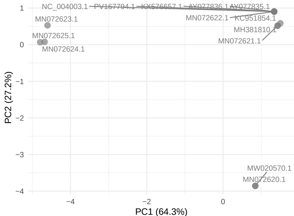
GTPV gene LSDV142
