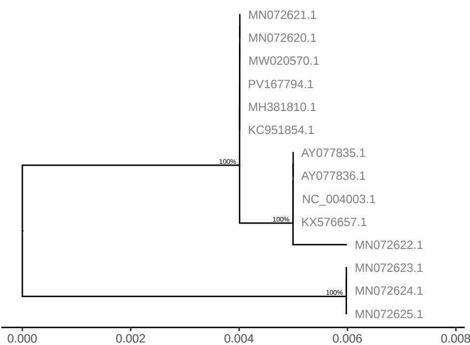
GTPV gene LSDV149
