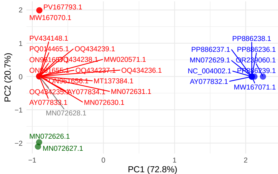
SPPV gene LSDV005
