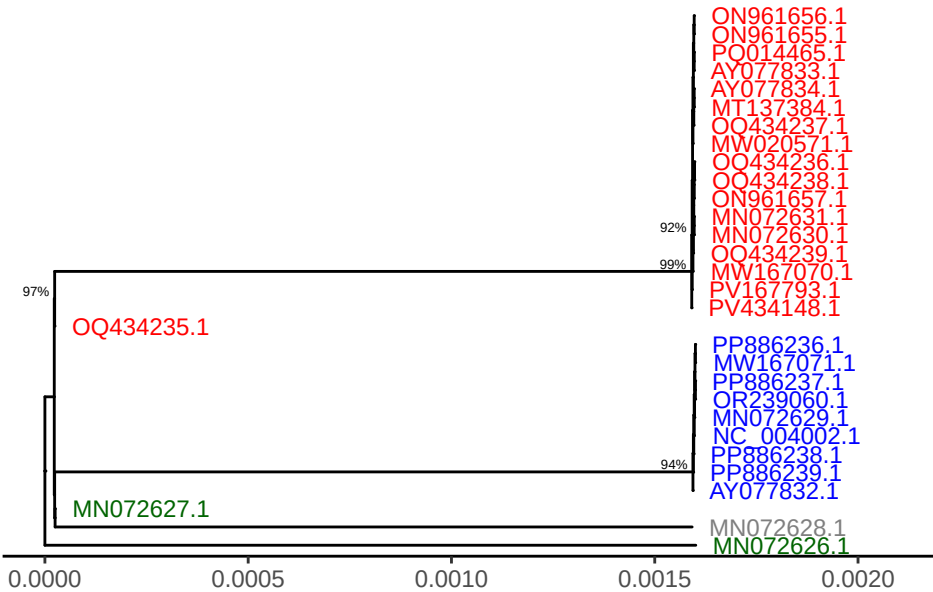
SPPV gene LSDV012
