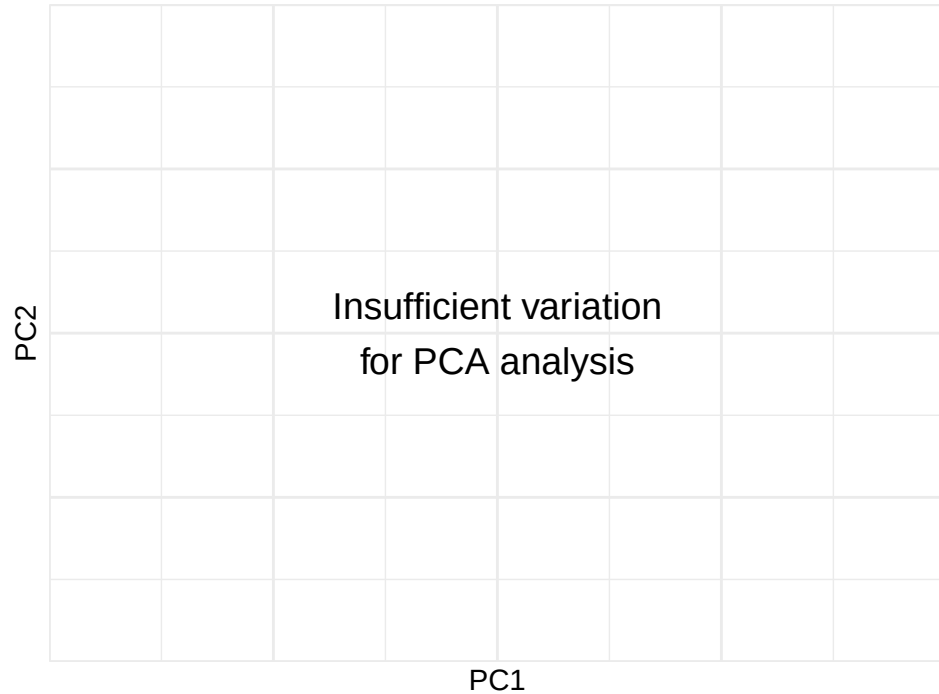
SPPV gene LSDV024
