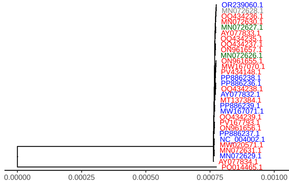
SPPV gene LSDV024
