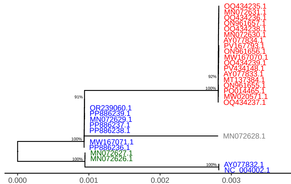
SPPV gene LSDV034
