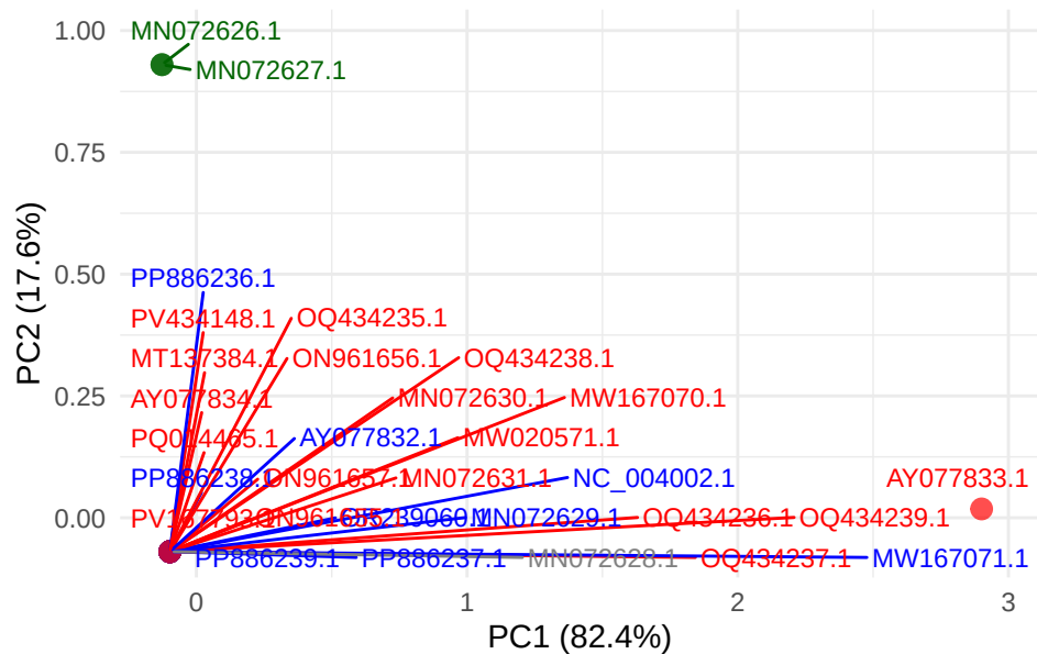
SPPV gene LSDV036
