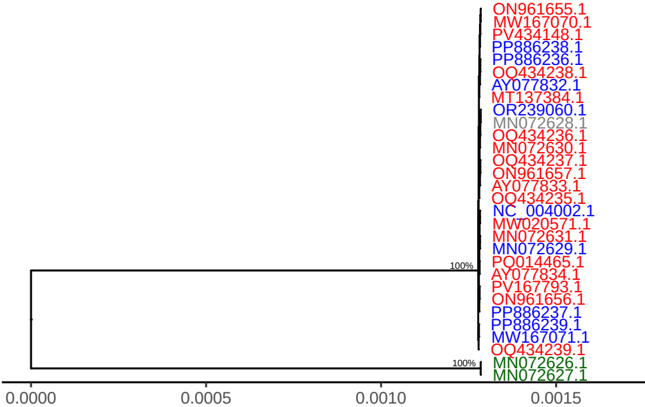
SPPV gene LSDV041
