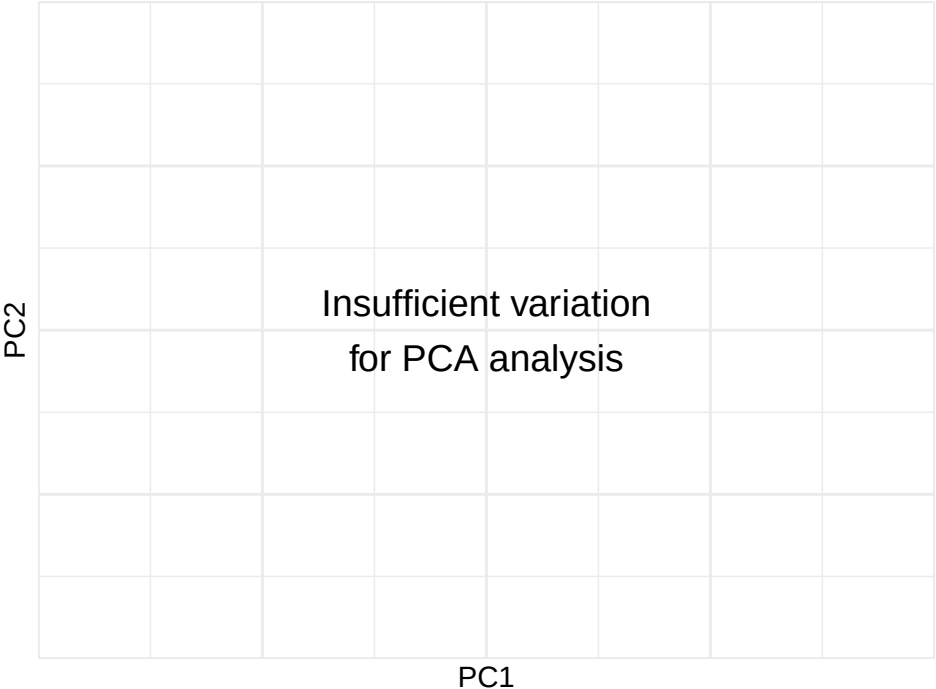
SPPV gene LSDV041
