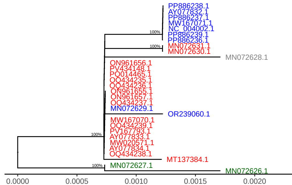
SPPV gene LSDV042
