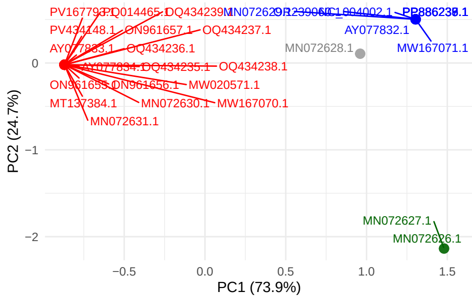
SPPV gene LSDV047
