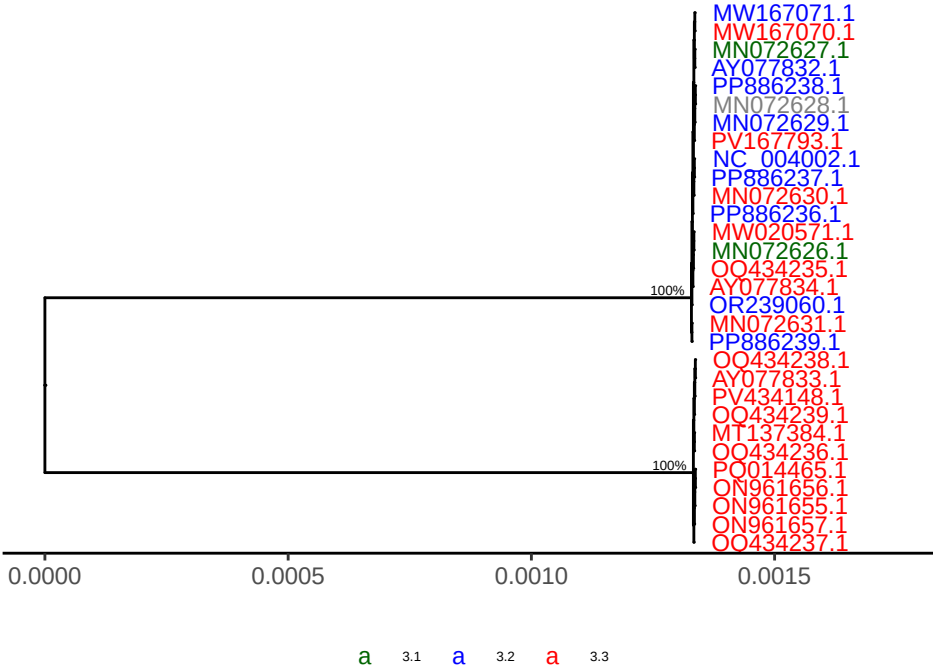
SPPV gene LSDV053
