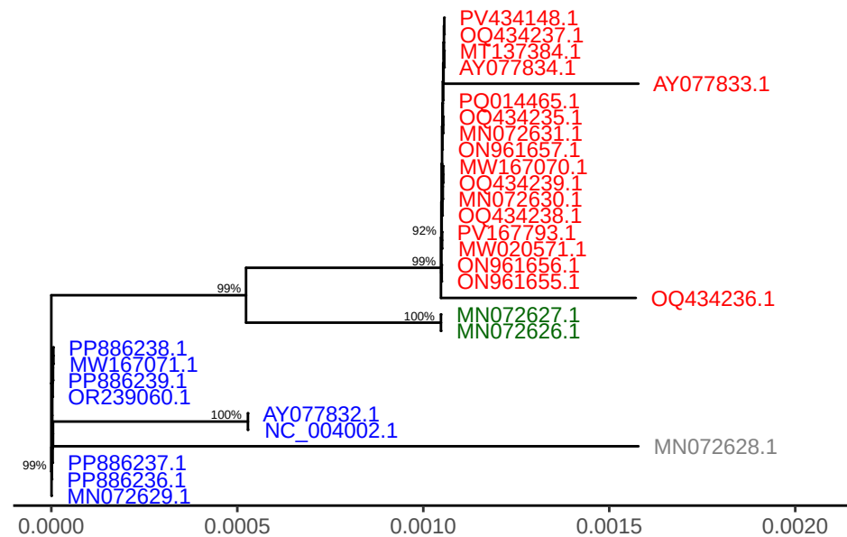
SPPV gene LSDV084
