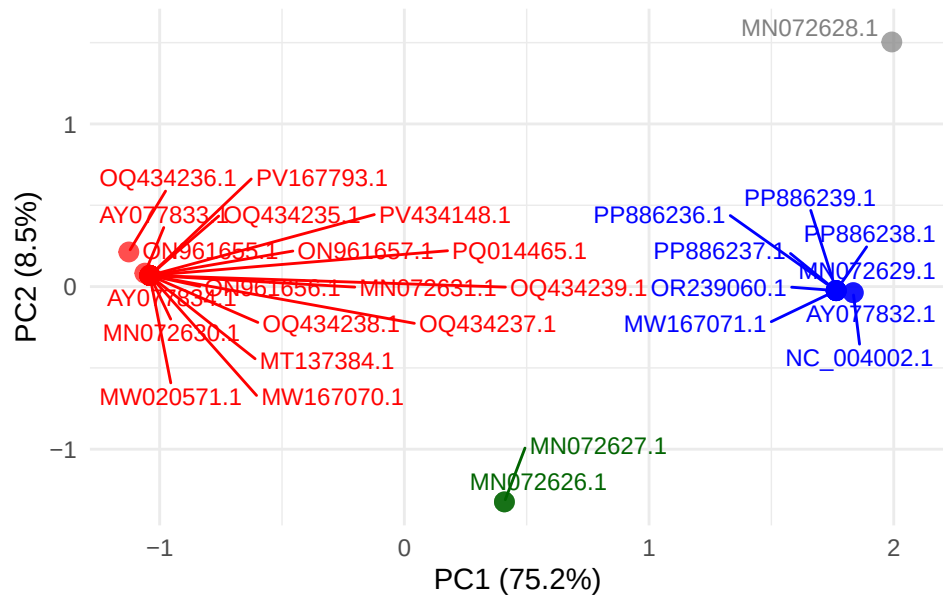
SPPV gene LSDV084
