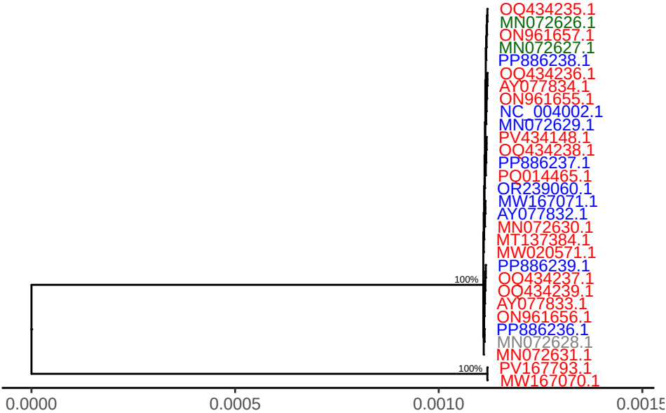
SPPV gene LSDV091
